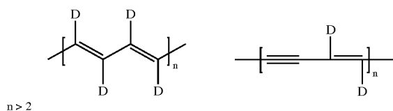
Scheme 1. Linear conjugated organic compounds and polymers
