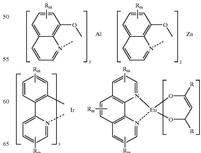
Scheme 4. Metal complexed organo-metallic compounds.
