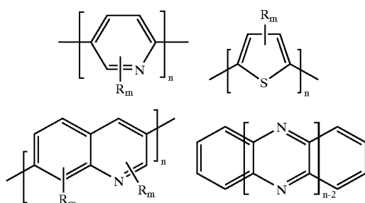
Scheme 3. Heterocyclic/fused ring heterocyclic combination.
